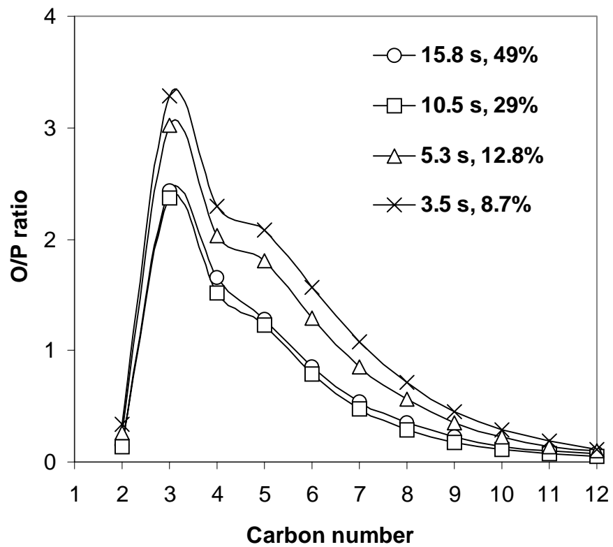
Figure 2.5. Space velocity effect on a -olefin to n -paraffin ratio (12.7 wt% Co/SiO 2 , 200°C, 20 atm, H 2 /CO = 2.0)
