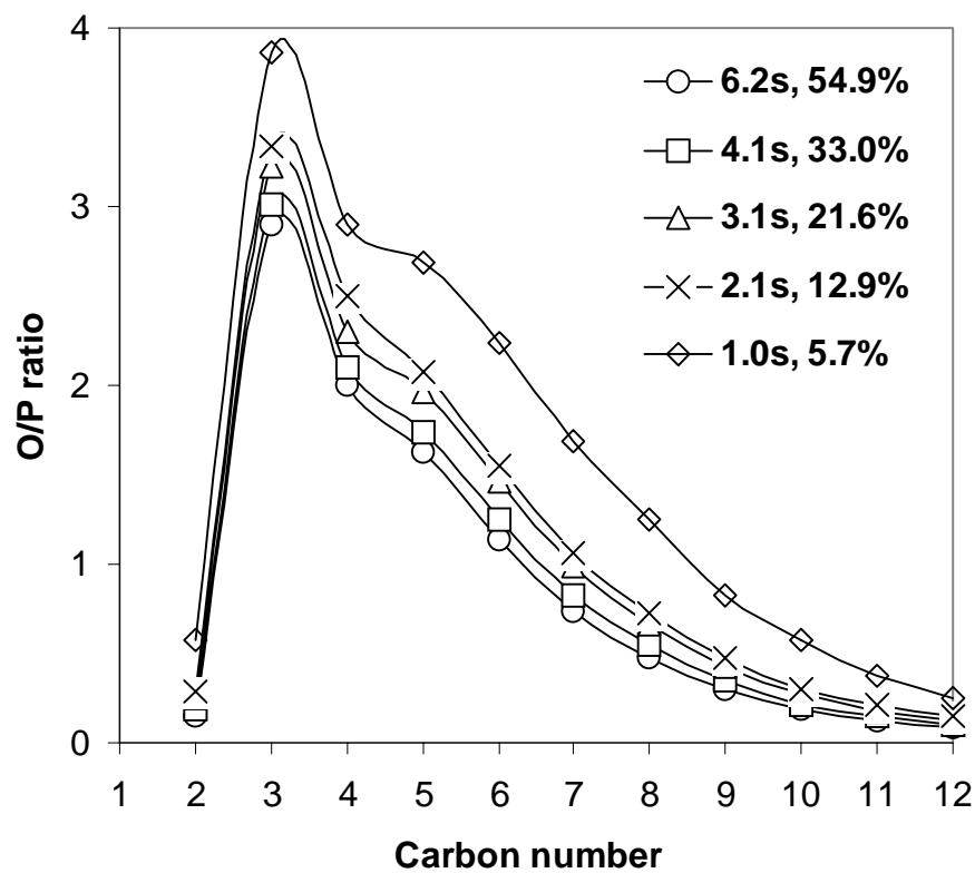
Figure 2.8. Space velocity effect on a -olefin to n -paraffin ratio (21.9 wt% Co/SiO 2 , 200°C, 20 atm, H 2 /CO = 2.0)
