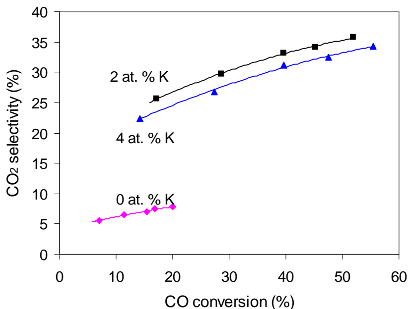
Fig. 1.11. CO 2 selectivity as a function of CO conversion on the catalysts (Zn/Fe = 0.1, 1 at.% Cu) with various potassium loading levels at 235 °C and 21.4 atm, H 2 /CO=2.
