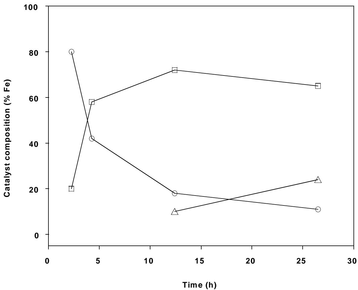
Figure 1. Phase composition changes of 100Fe/4.6Si/2.7Cu/1.0K catalyst during activation with H 2 at 220°C, 0.1 MPa. (○), superparamagnetic oxide; (□), Fe 3 O 4 ; (△), Fe 0 .
