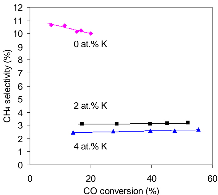
Fig. 1.12. Methane selectivity as a function of CO conversion on the catalysts ( Zn/Fe = 0.1 , 1 at.% Cu) with various potassium loading levels at 235 °C and 21.4 atm, H_2/CO=2 .
