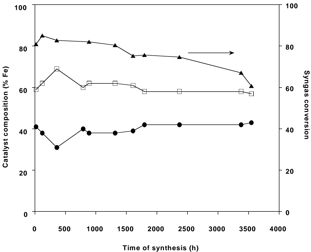
Figure 3. Long term phase composition of H 2 activated 100Fe/4.6Si/2.7Cu/1.0K catalyst during FT synthesis (270°C, 1.3 MPa, H 2 /CO=0.7, whsv=3.1 sl h -1 g-Fe -1 ). (□), Fe 3 O 4 ; (●), ε'-Fe 2.2 C; (▲), syngas conversion.
