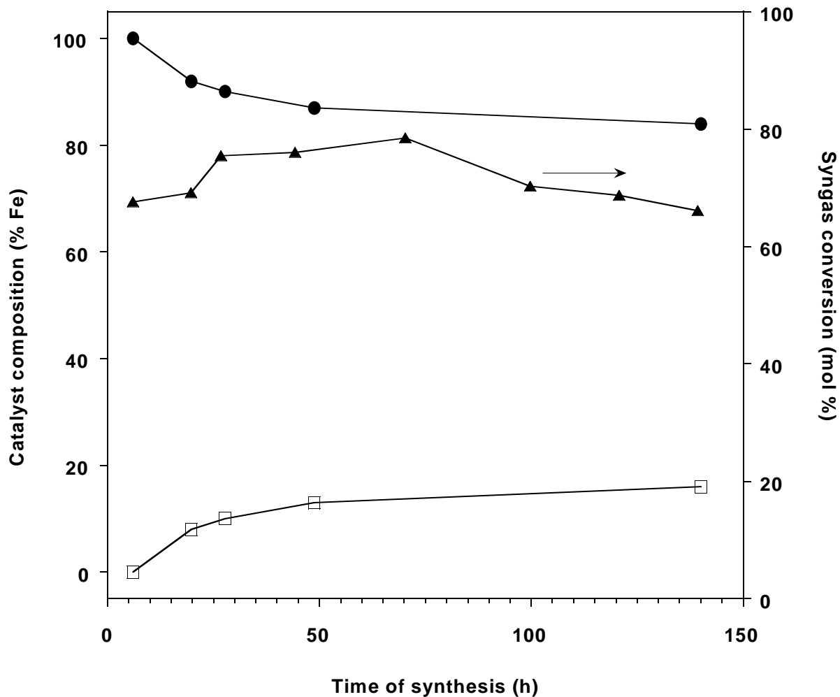
Figure 5. Phase composition of CO activated 100Fe/8.9Cu/1.9K/67kaolin catalyst during FT synthesis (270°C, 1.3 MPa, H 2 /CO=0.7, whsv=3.1 sl h -1 g-Fe -1 ). (●), \chi -Fe 3 C 2 and superparamagnetic carbides; (□), Fe 3 O 4 ; (▲), syngas conversion. Data from reference 16.
